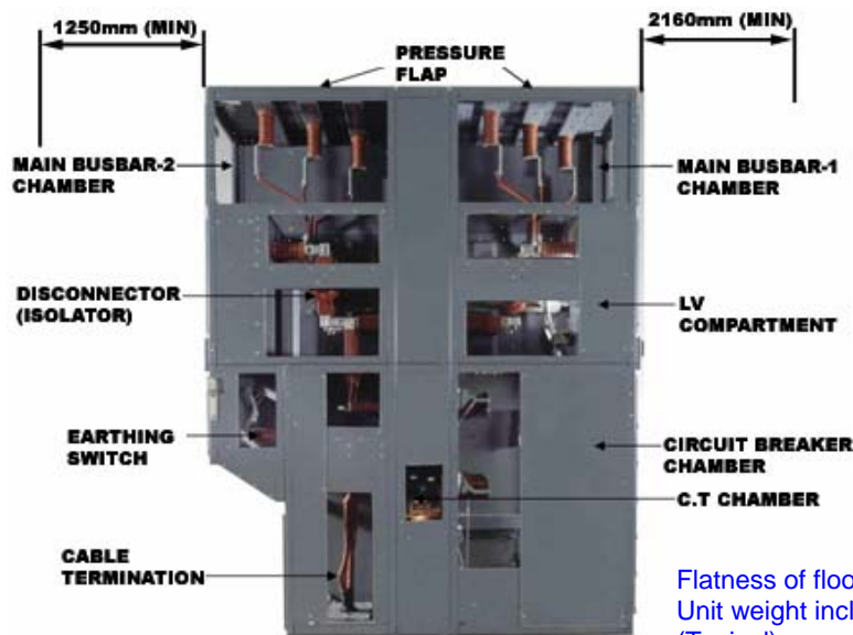
Typical cross sectional view Outgoing Panel
